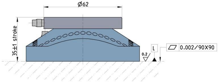
air bearing with piston AL-90-71-HD+K
